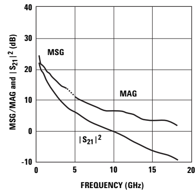
Figure 24. MSG/MAG and |S_{21}|^2 vs. Frequency at 4V, 40 mA.
